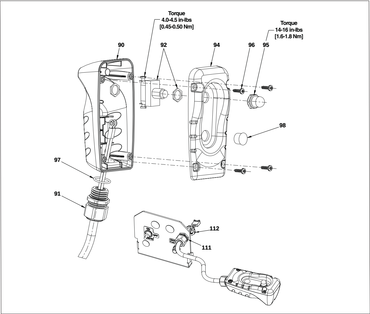
Figure 5, Pendant Assembly
