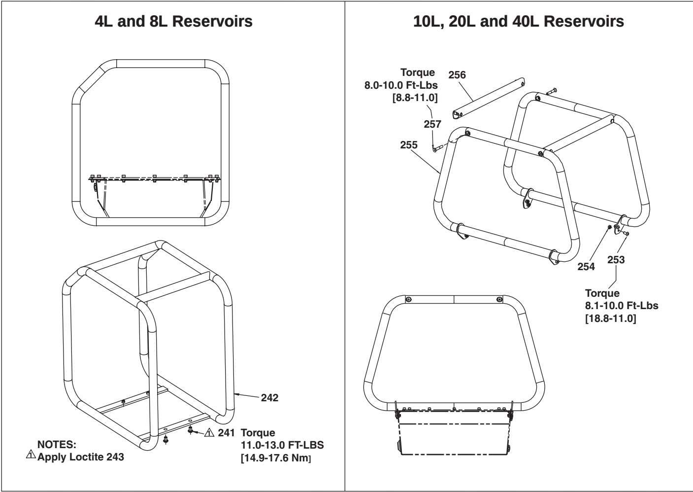
Figure 7, Roll Bar Assembly (optional accessory)
