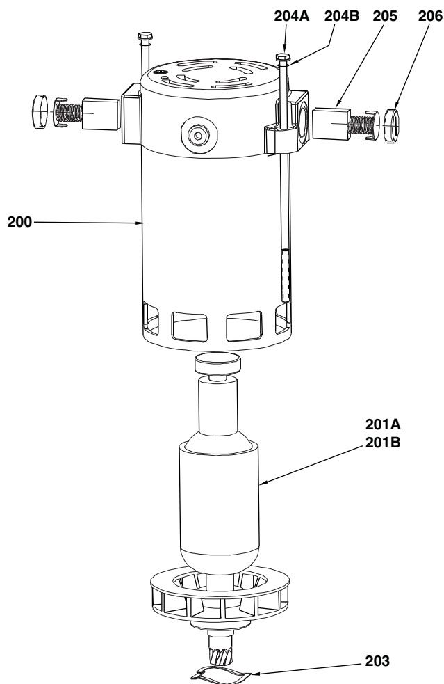
Figure 6, Motor Assembly, Universal
