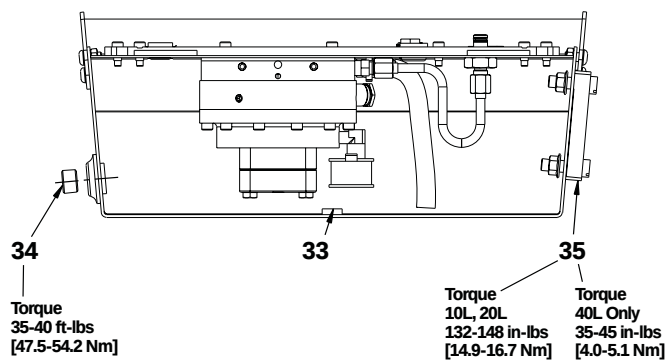
Figure 1, Reservoir Assembly
