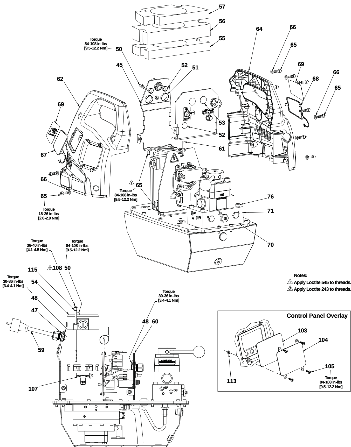
Figure 2, Pump Assembly
