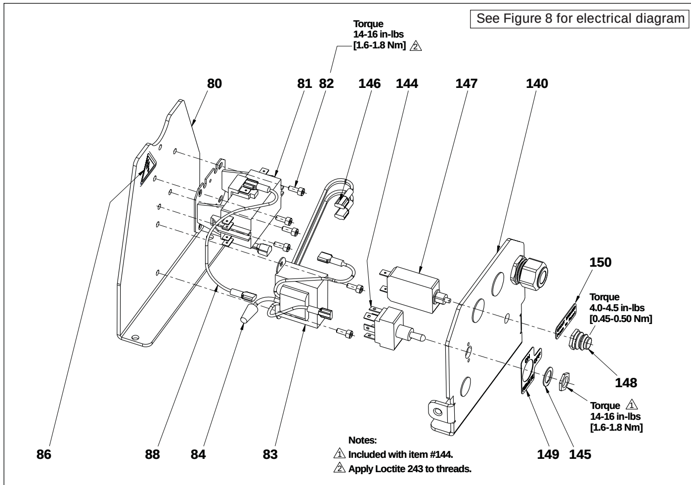
Figure 4, Front and Mid Bracket Assemblies
